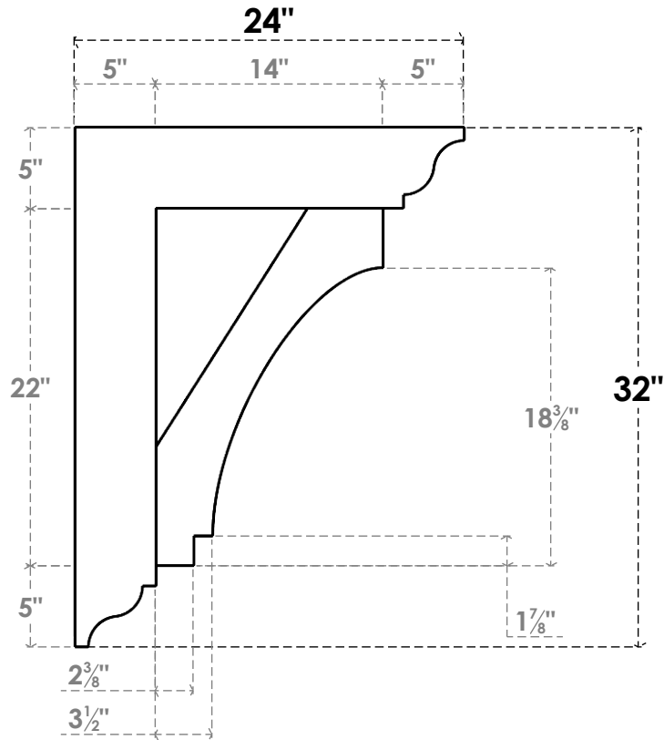
SIDE PROFILE
