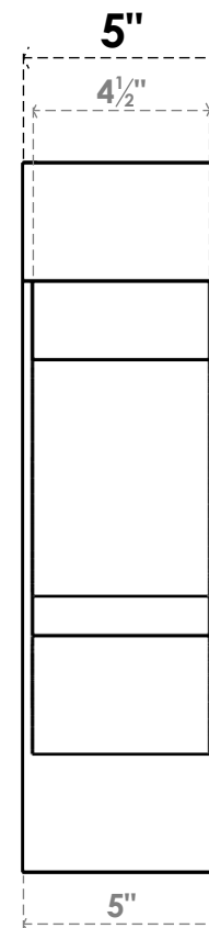
FRONT PROFILE
