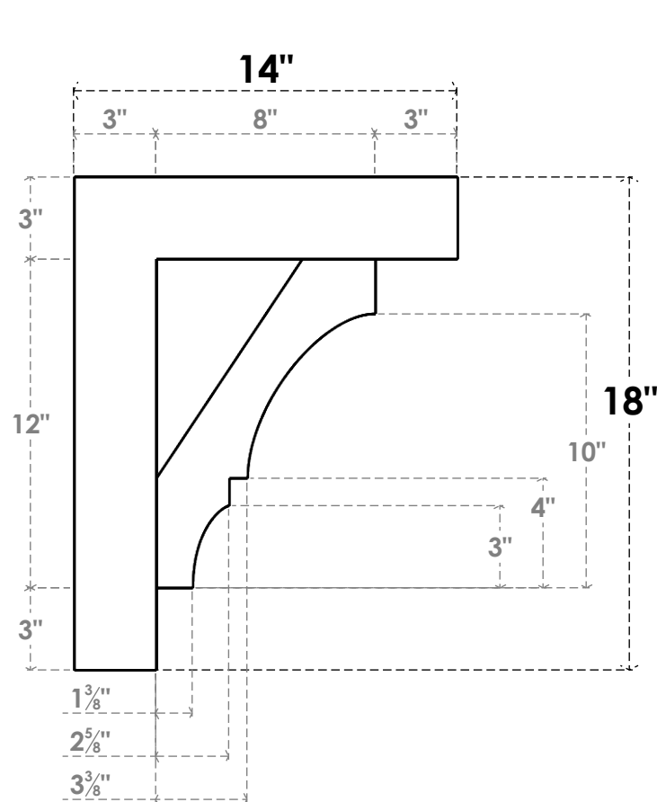
SIDE PROFILE
