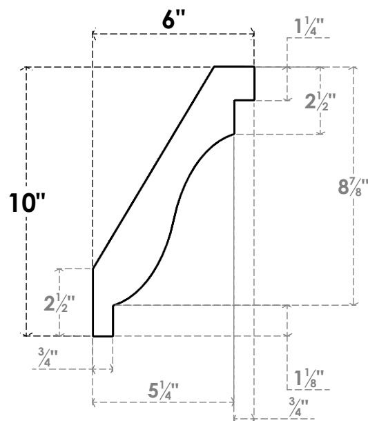
SIDE PROFILE
