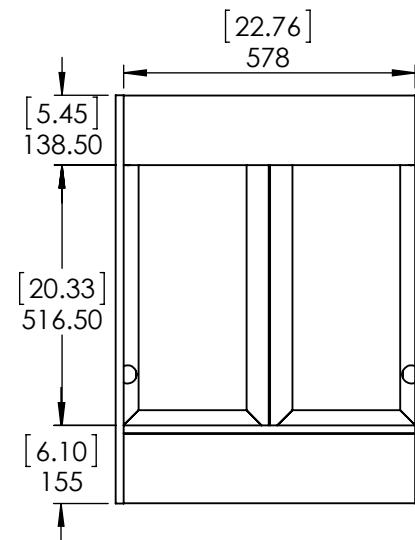
BACK VIEW
