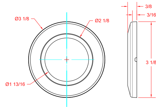
ICSS-CCR-COVER Detail
