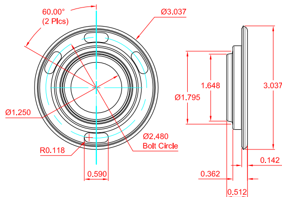
IFSS-CER-FLANGE Detail
