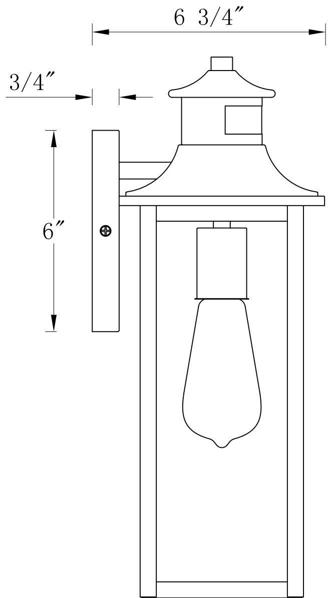
SIDE VIEW
