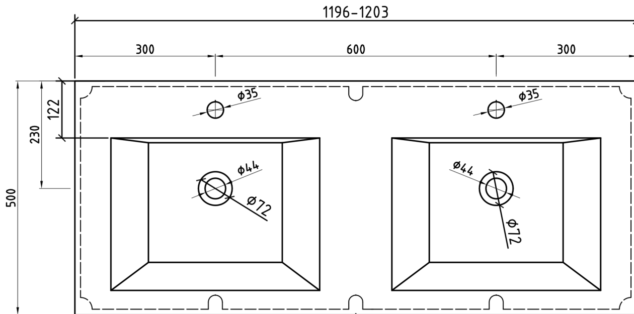
SECTION B-B
