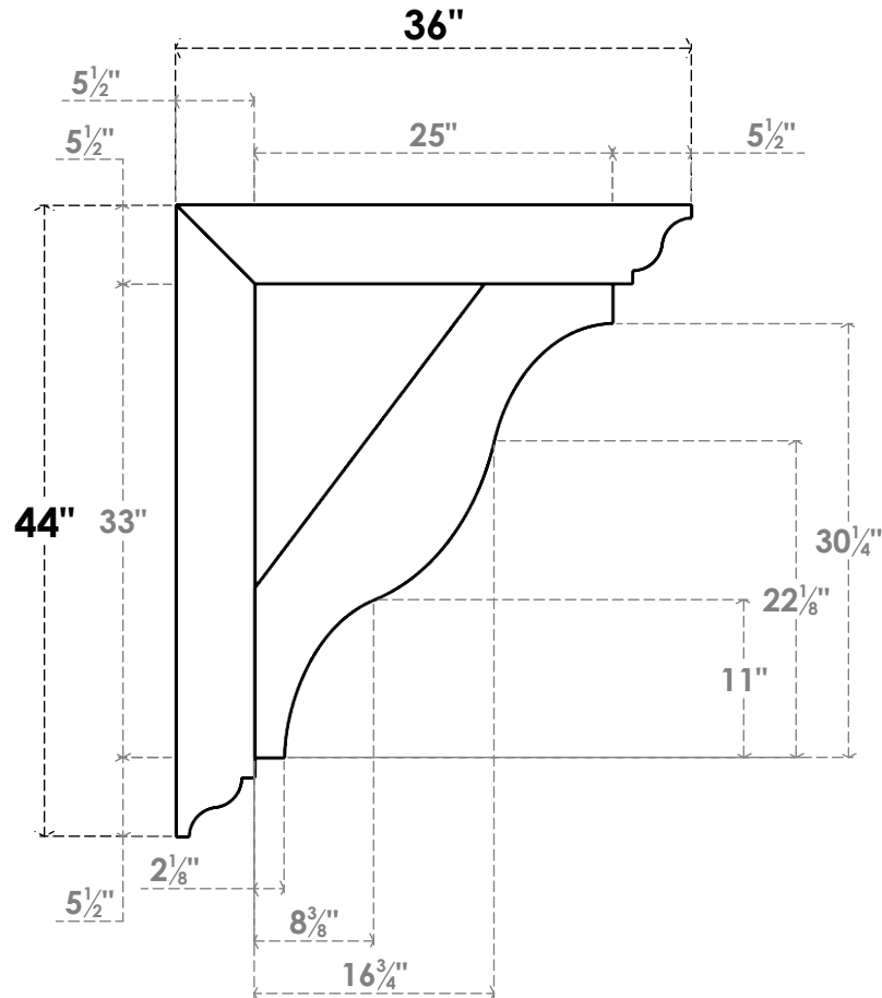
SIDE PROFILE
