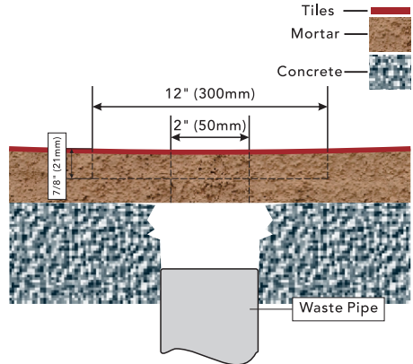
Floor Cross-Section Diagram
