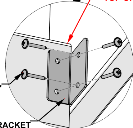
797 (x8) SCREW - 1"
