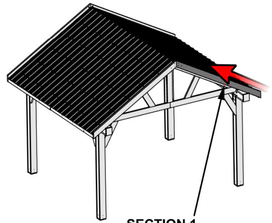
SECTION 1 ROOF ASSEMBLY 'A'
