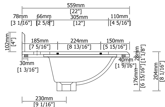
RIGHT VIEW
