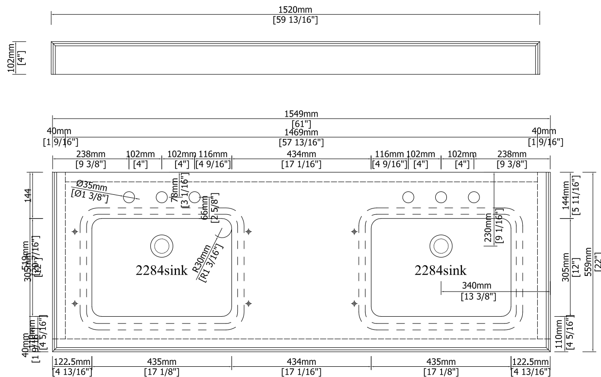
TOP VIEW
