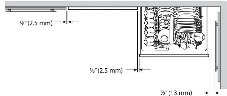
Minimum clearances (inches (mm))
