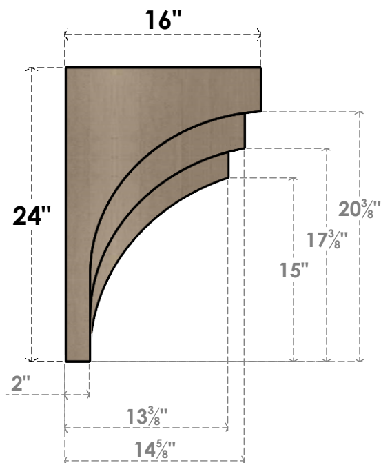
SIDE PROFILE
