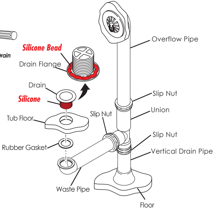
Fig. 1 - Securing Your Drain
