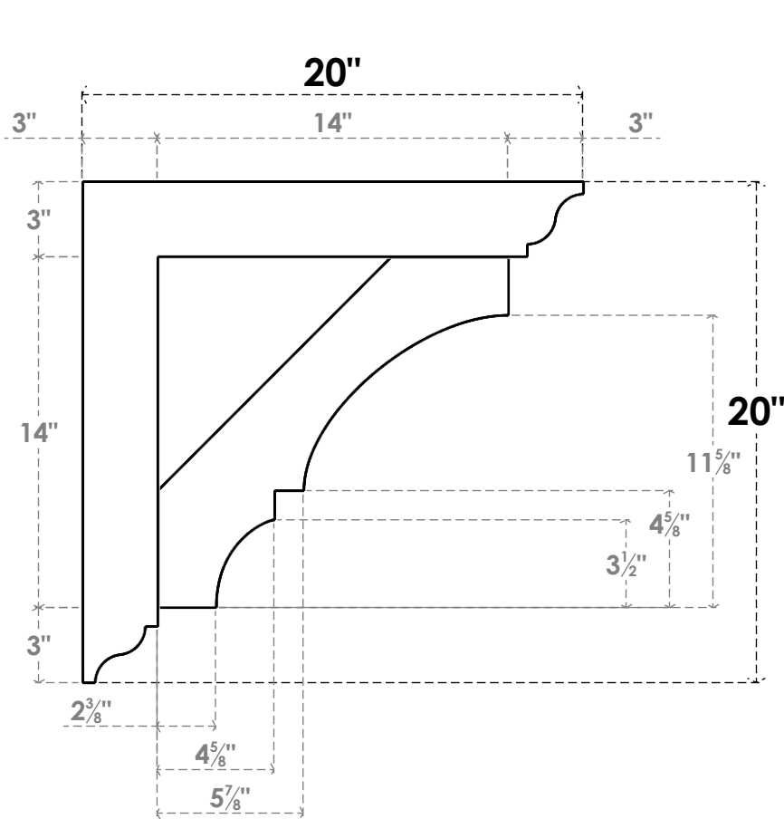
SIDE PROFILE
