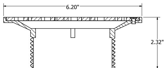
SECTION A-A SCALE 1
