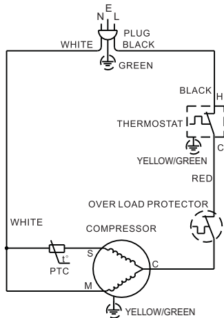
CIRCUIT DIAGRAM
