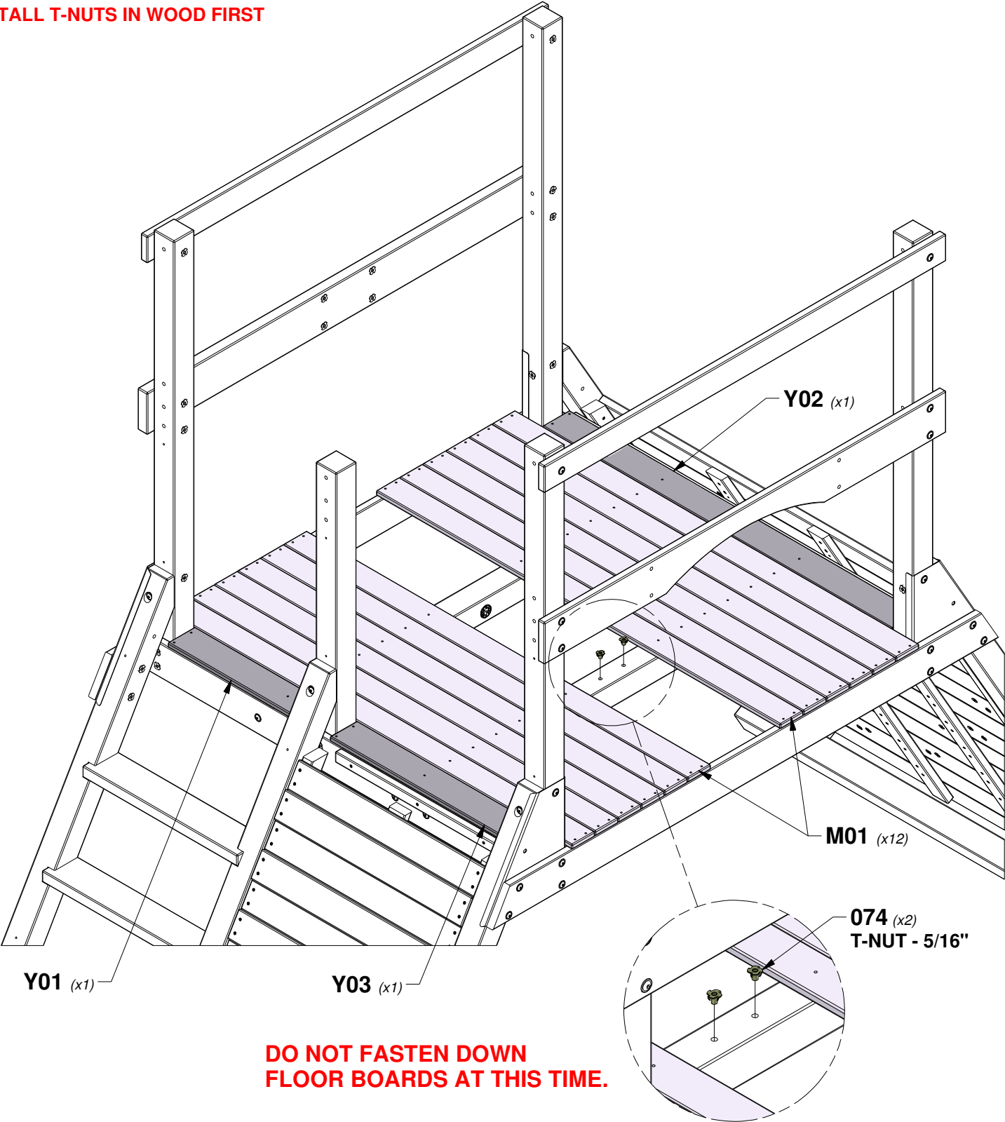
Y02 | FLOOR BOARD - W4L15745 (x1) | 5/8"x4"x51 1/2" (16x102x1307)
