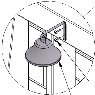
392 (x2) SCREW - 3/4"
