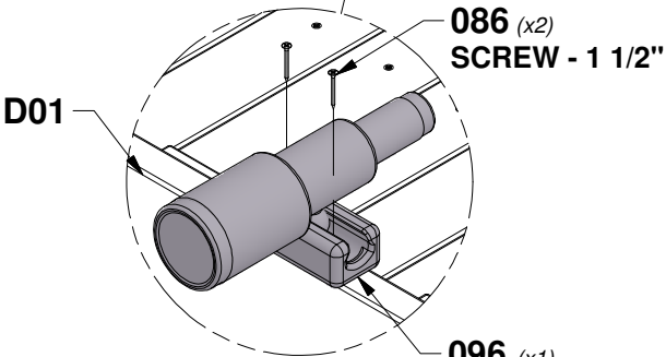
096 (x1) TELESCOPE CENTER IN D01 BOARD
