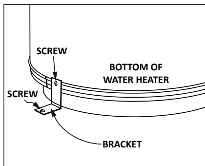
Figure 16: Water Heater Bracket and screws.
