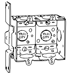
LXWV-2G 2-gang with "CV" bracket recessed 7/8"
