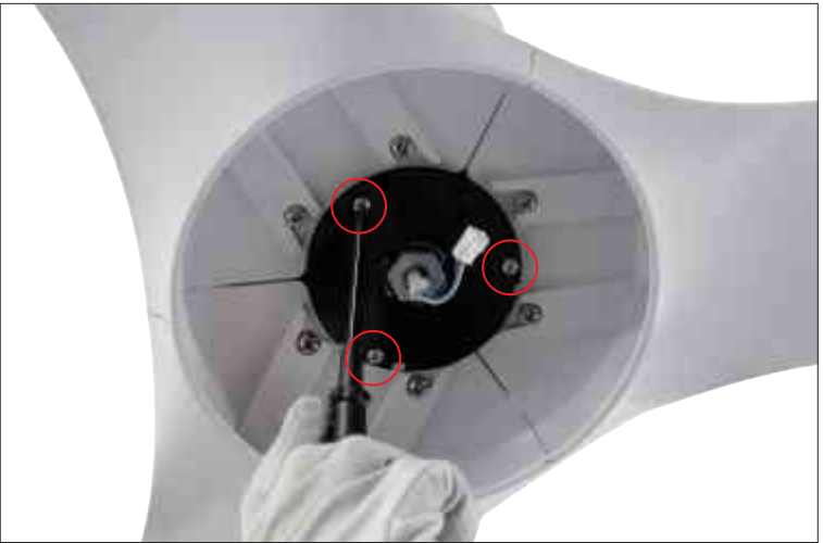
Step 17 Remove the three screws which are used to install the light plate.
