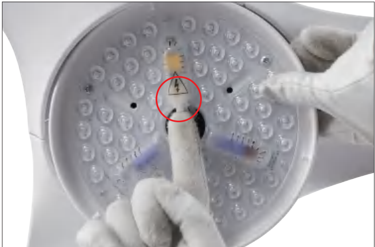
Step 18 Connect the cord to light source.
