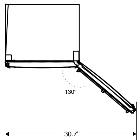
TOP OF REFRIGERATOR WITH DOORS OPEN 130°
