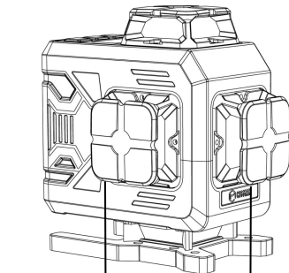
Side Vertical Laser Window
