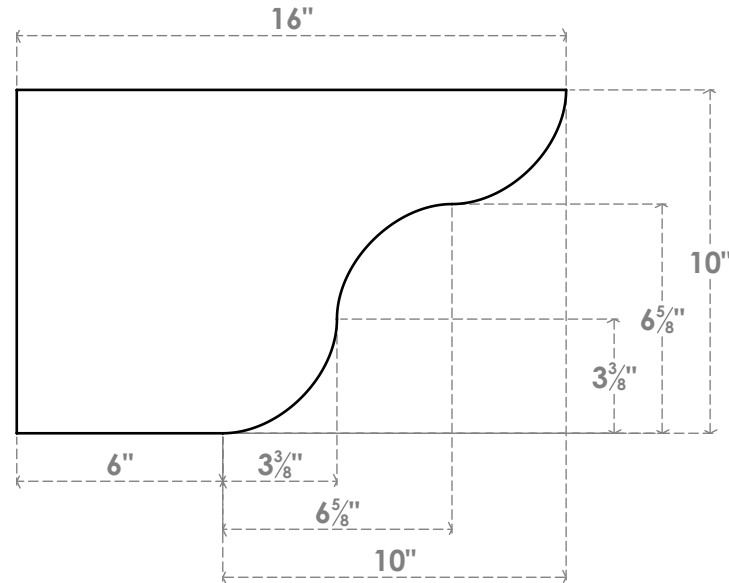
SIDE PROFILE
