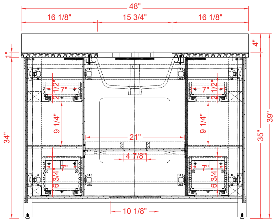
BACK VIEW
