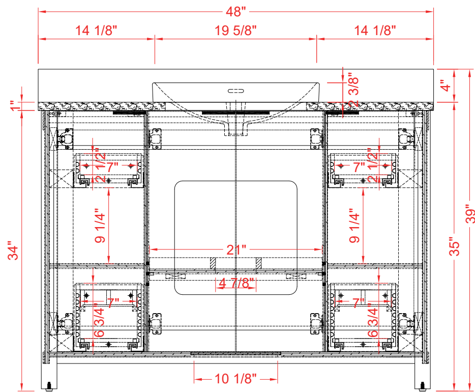
BACK VIEW
