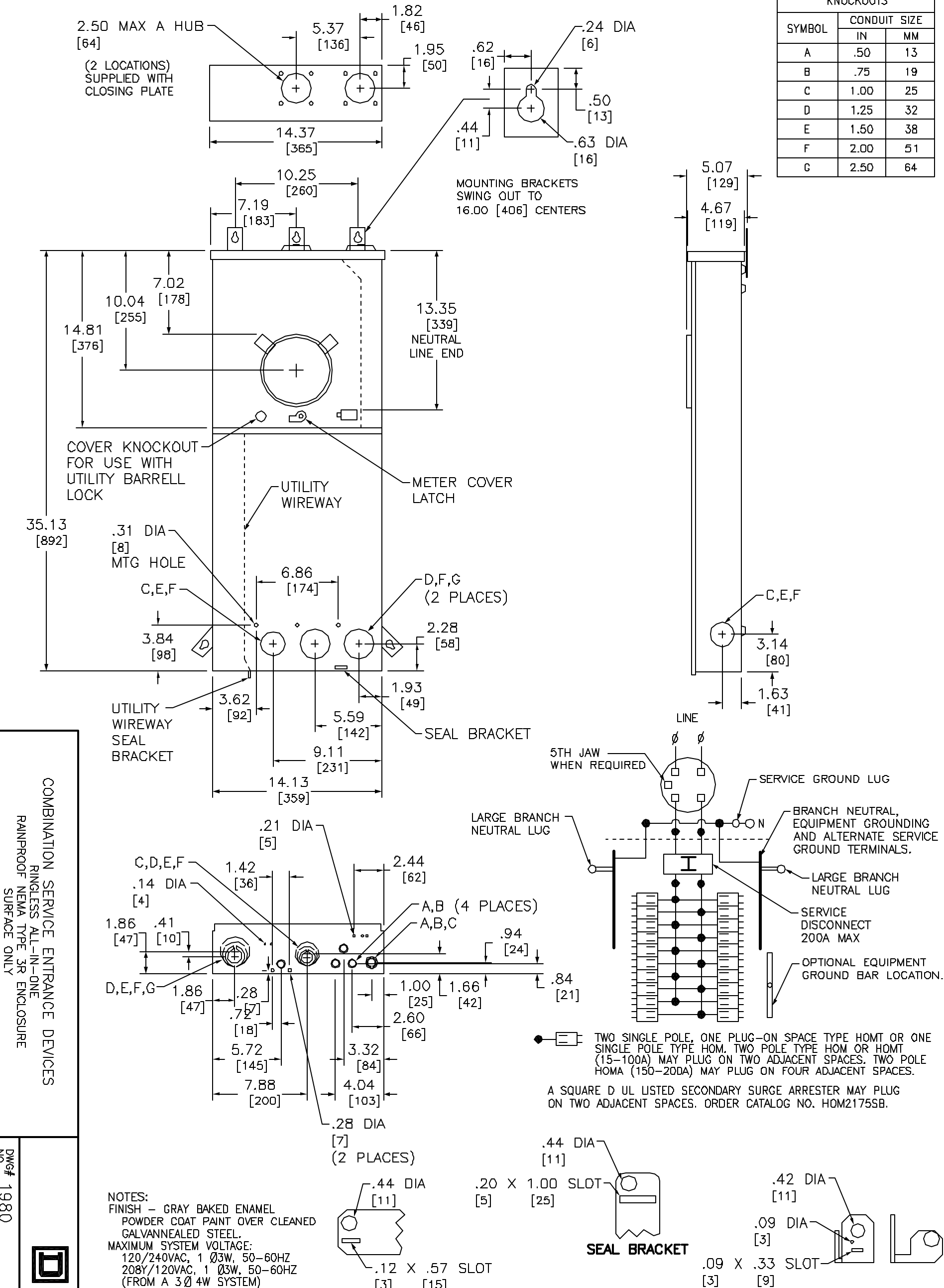
UTILITY WIREWAY SEAL BRACKET
