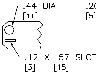
UTILITY WIREWAY SEAL BRACKET
