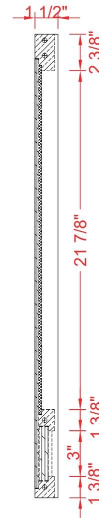
SIDE VIEW
