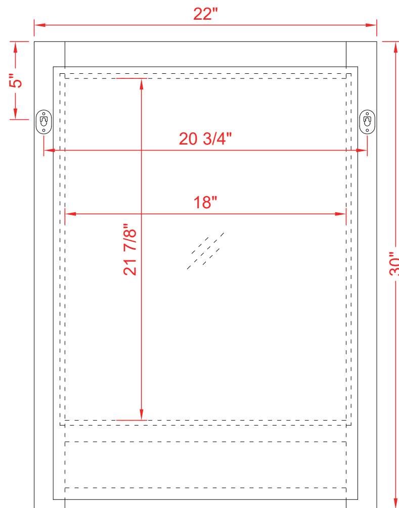
BACK VIEW
