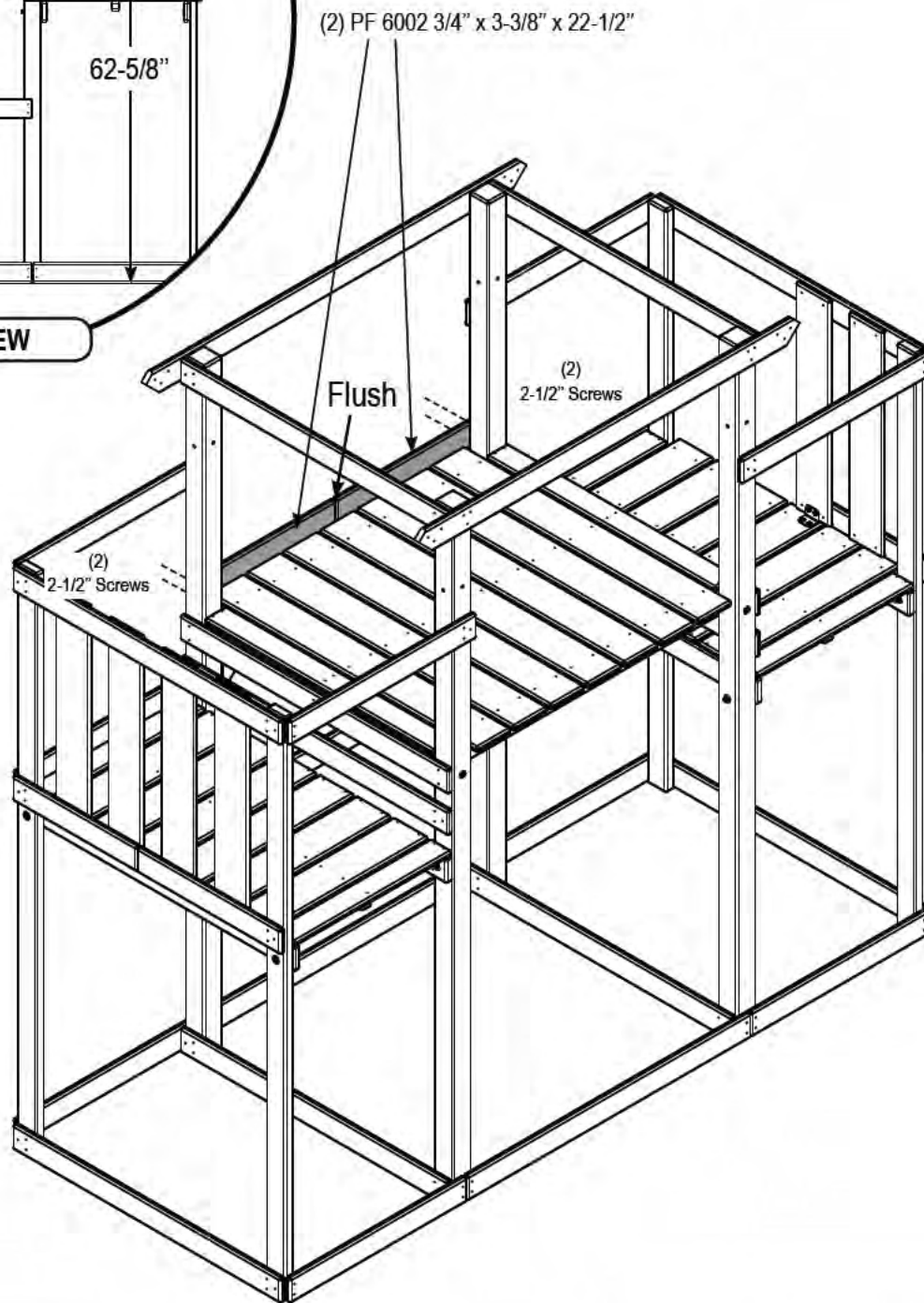
2-1/2" Deck Screw (x4)
