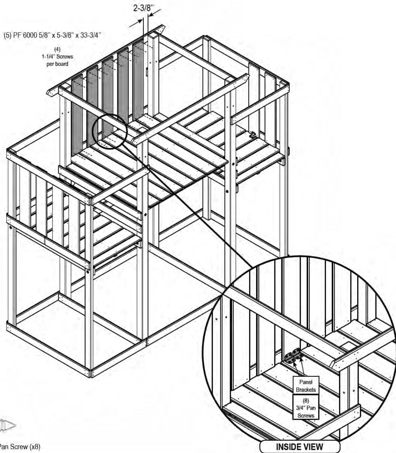
1-1/4" Deck Screw (x20)
