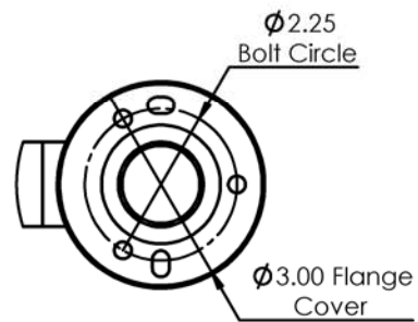
Flange Detail A
