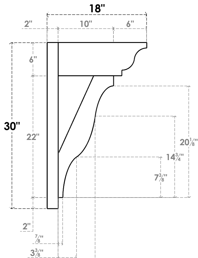
SIDE PROFILE
