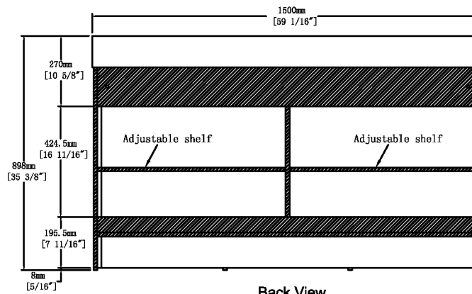
Back View
