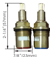
Cartridge (Type J)
