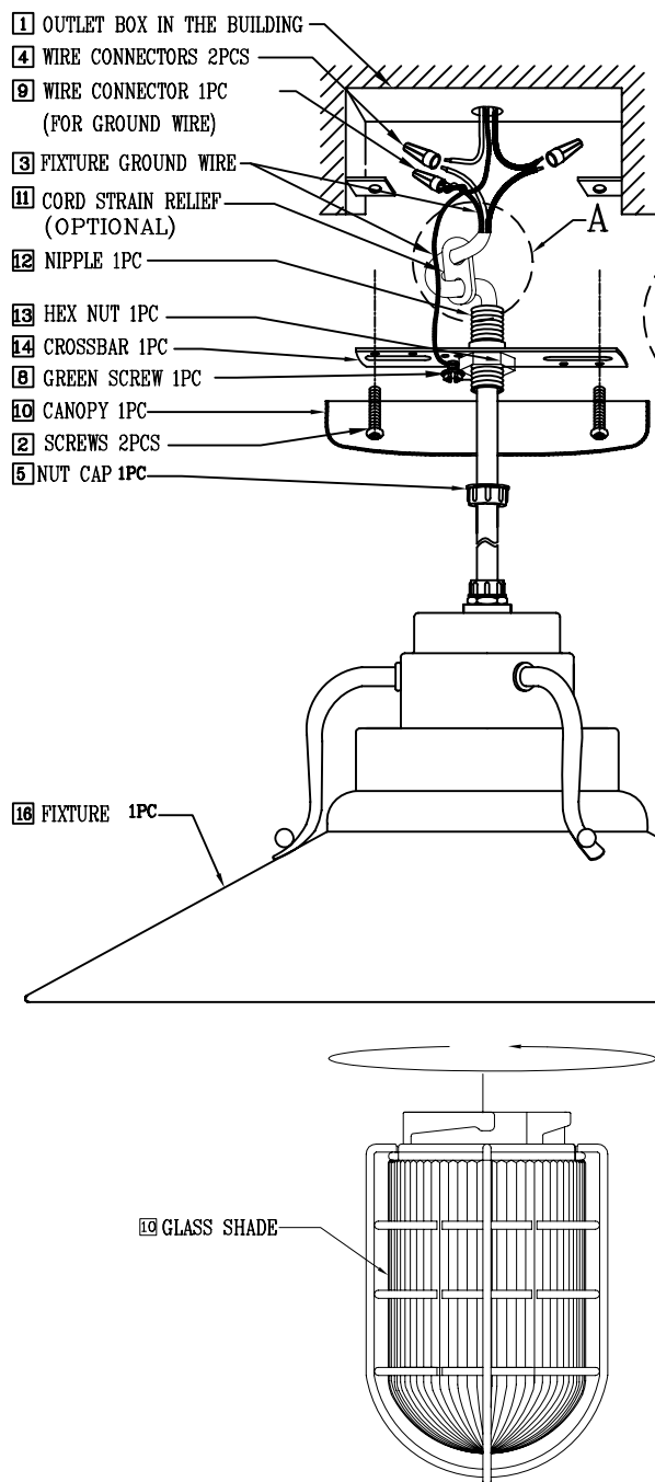
INSTALLING FIGURE
