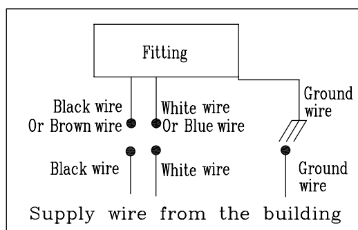
Circuit diagram 1
