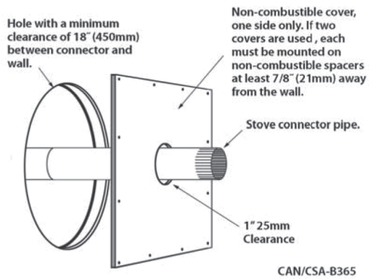
Figure 4 ONLY APPROVED CANADIAN WALL PASS THROUGH
