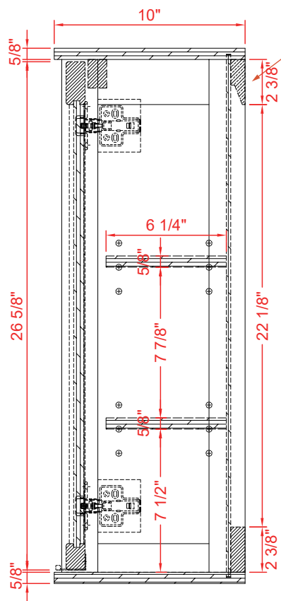
SIDE VIEW
