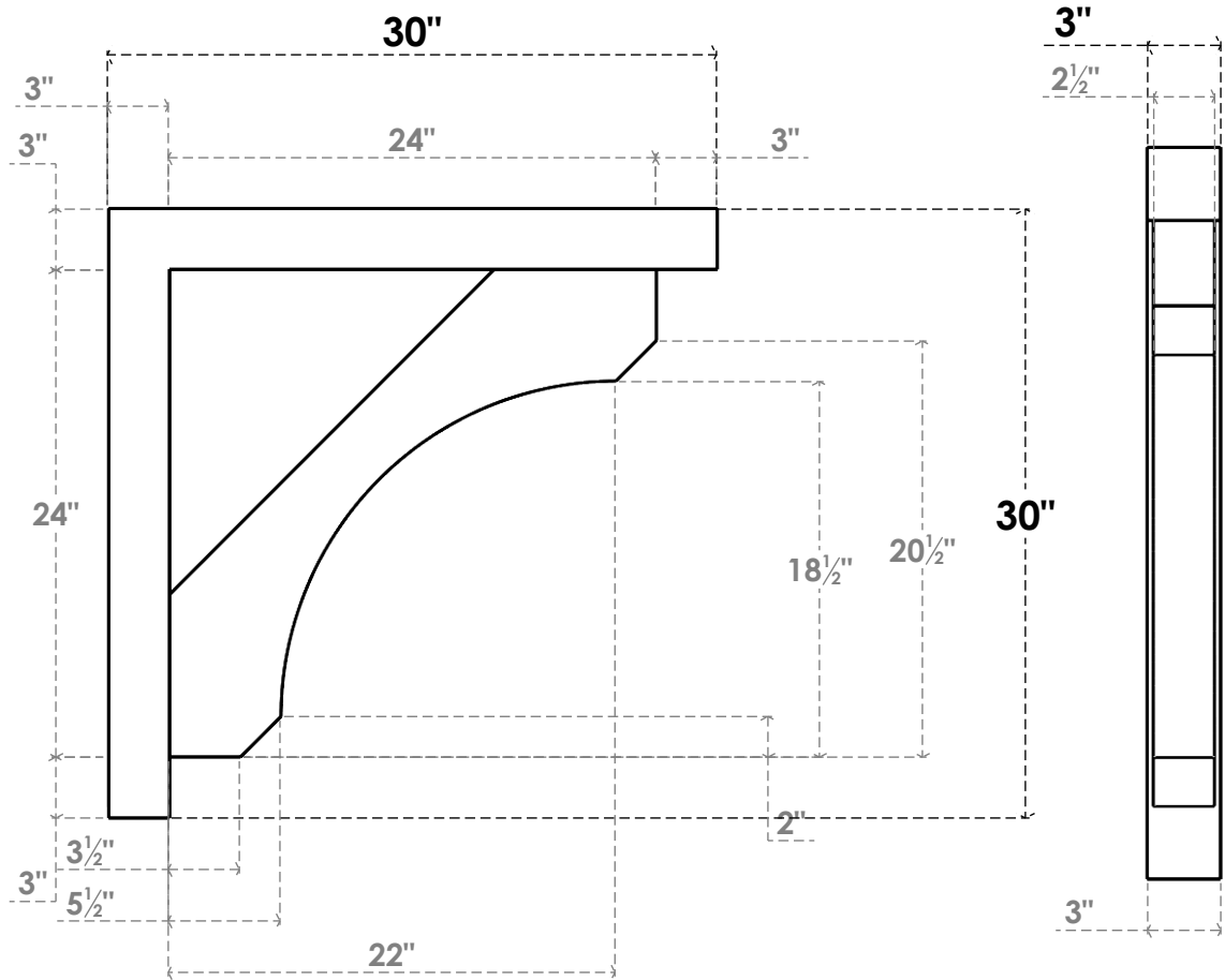
SIDE PROFILE
