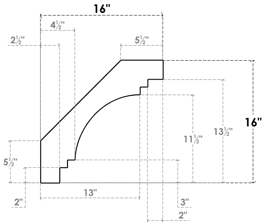
SIDE PROFILE
