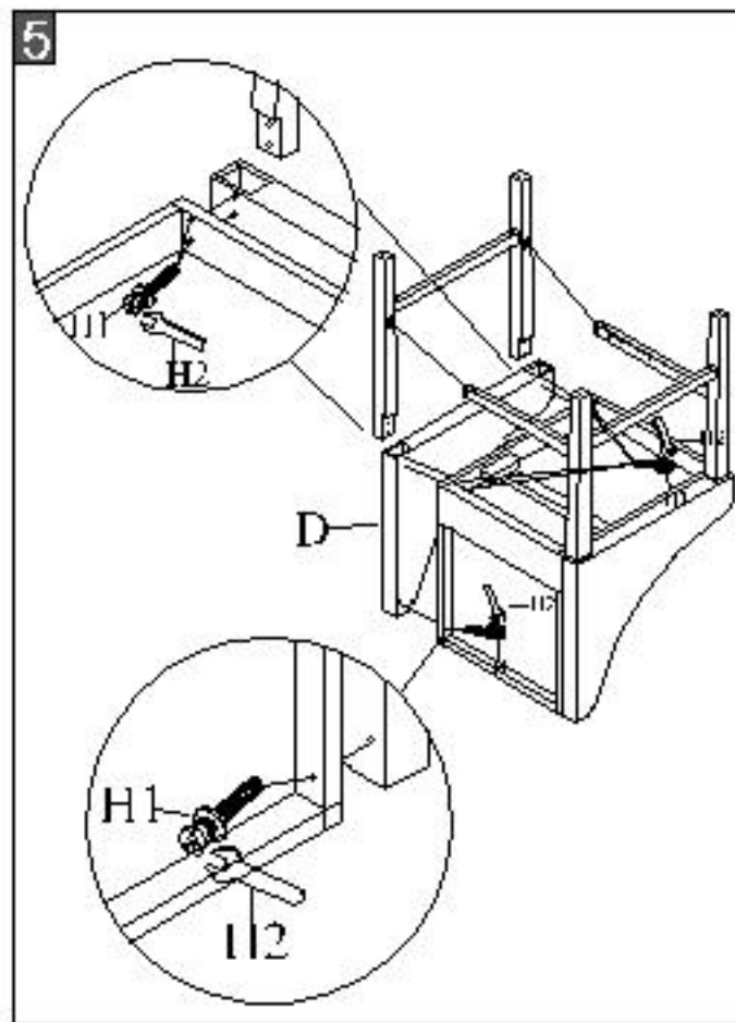
Step 5: Attach the assembled left legs (F&H) to left armrest(D) together with front / back stretchers (K&L). Then,assemble left armrest (D) with seat cushion (B).Using L-wrench (H2) to lock with 5*bolts (H1).
