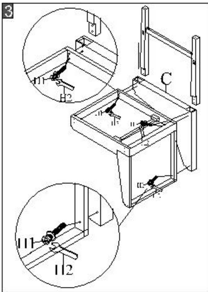
Step 3: Attach the assembled right legs (E&G) to right armrest(C).Then assemble right armrest (C) with seat cushion (B). Using L-wrench (H2) to lock with 5*bolts (H1).
