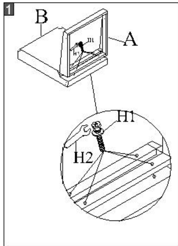
Step 1: Assemble seat cushion (B) with chair back (A).Using L-wrench (H2) to lock with 4*bolts (H1).
