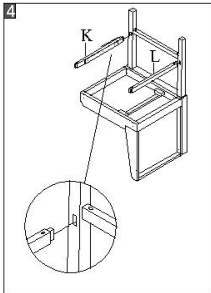
Step 4: Assemble front stretcher (K) with R/front leg (E). Then, assemble back stretcher (L) with R/back leg (H).
