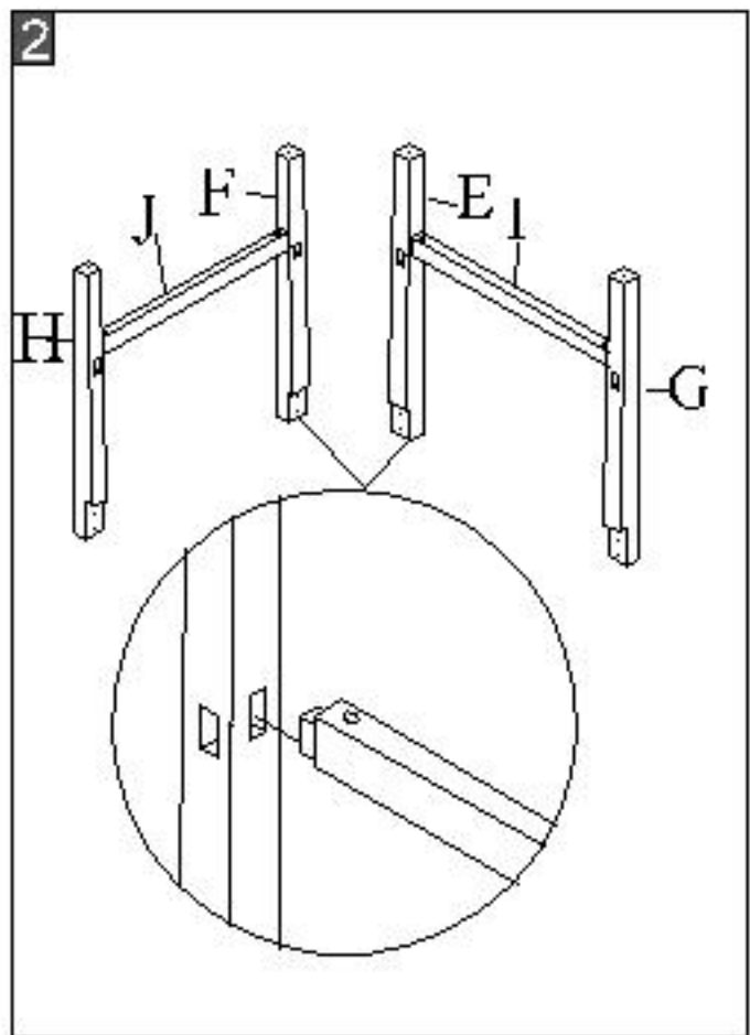
Step 2: Assemble legs (E & G) with R/stretchers (I). Then, assemble legs (F&H) with L/stretchers (J).
