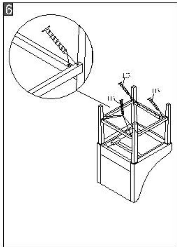
Step 6: Lock the stretchers tight with legs by using 8*screws (H3).
