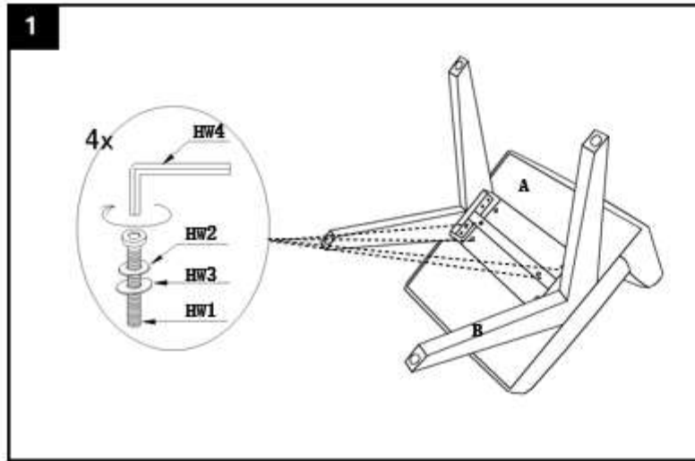
Step 1: attach base B to seat A with HW1, HW2 and HW3
