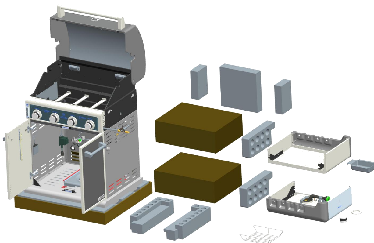
Exploded View of Main Components
