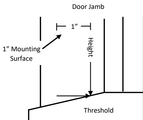
Diagram 2- Threshold Side View
