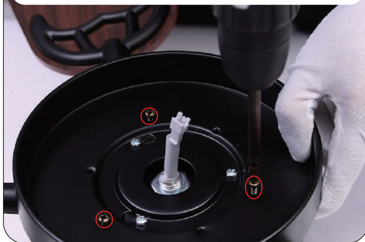
10. Remove the three light kit screws on light plate
