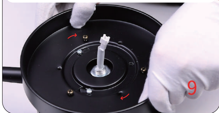
8. Feed the wire plugs through the center hole. Wrap keyhole slots around the screws and twist clockwise
