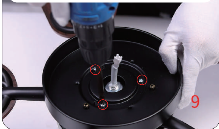
9. Insert the third light kit screw, and then tighten all three light kit screws
