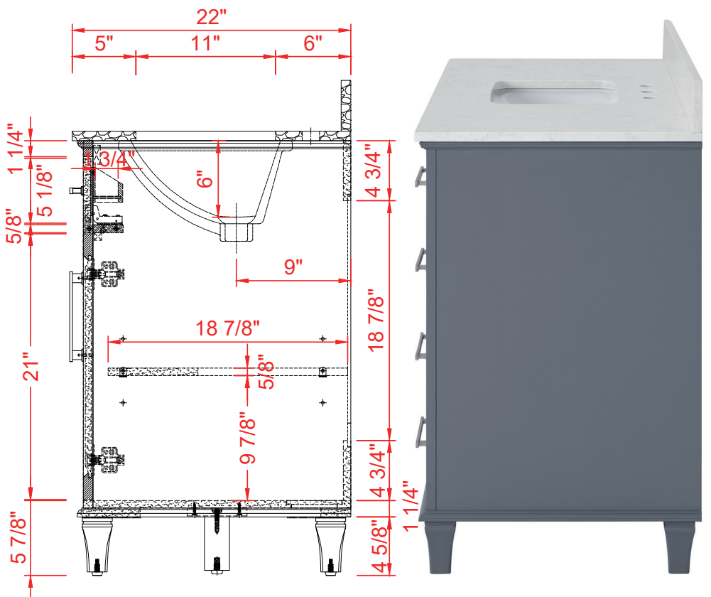
SIDE VIEW
