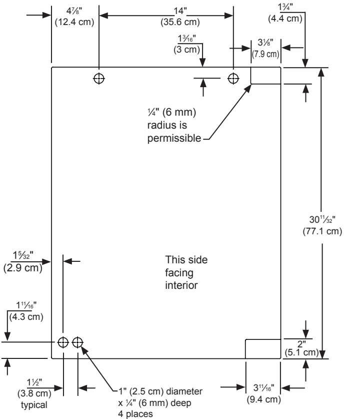
Figure 19 Left Hand Hinged Door 24" (61 cm) wide appliance
