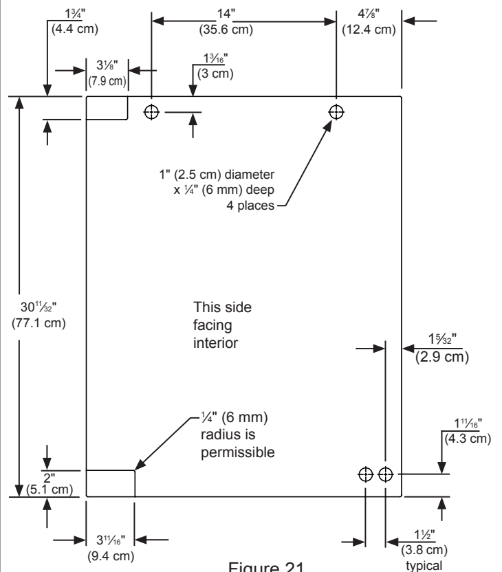
Figure 21 Right Hand Hinged Door 24" (61 cm) wide appliance
