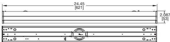
2 ft. Dimensions
