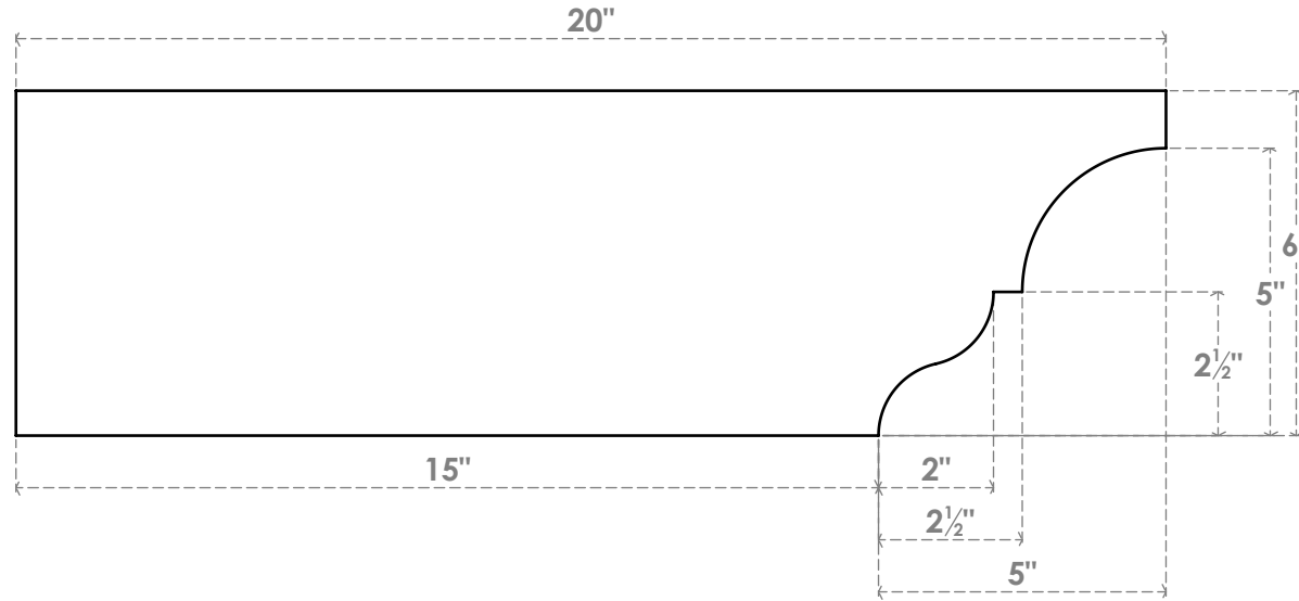
SIDE PROFILE
