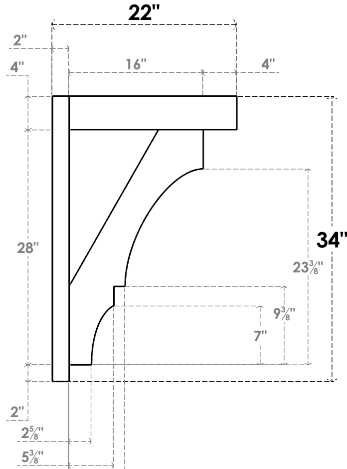
SIDE PROFILE
