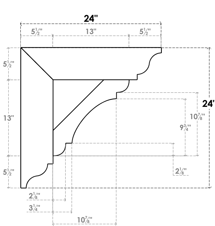
SIDE PROFILE
