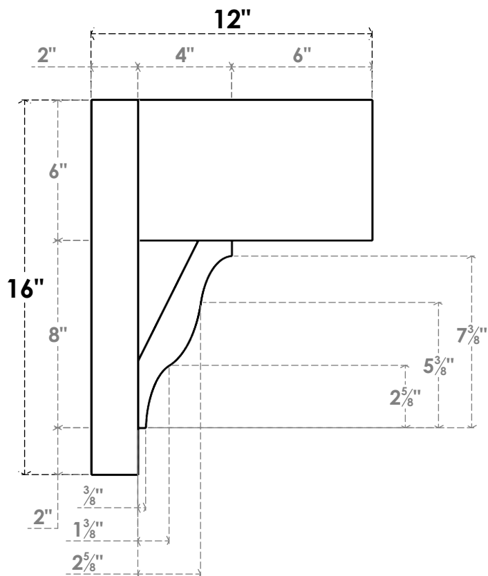
SIDE PROFILE
