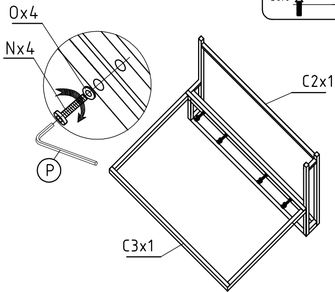
Step 8
